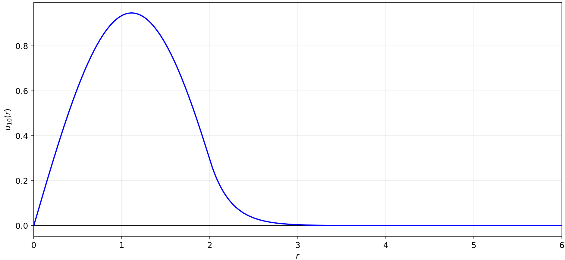
Reduced Radial Wave Function: n = 1, \ell = 0
