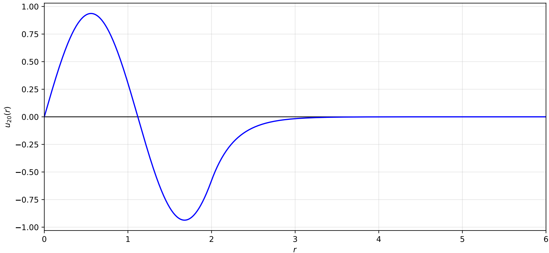
Reduced Radial Wave Function: n = 2, \ell = 0
