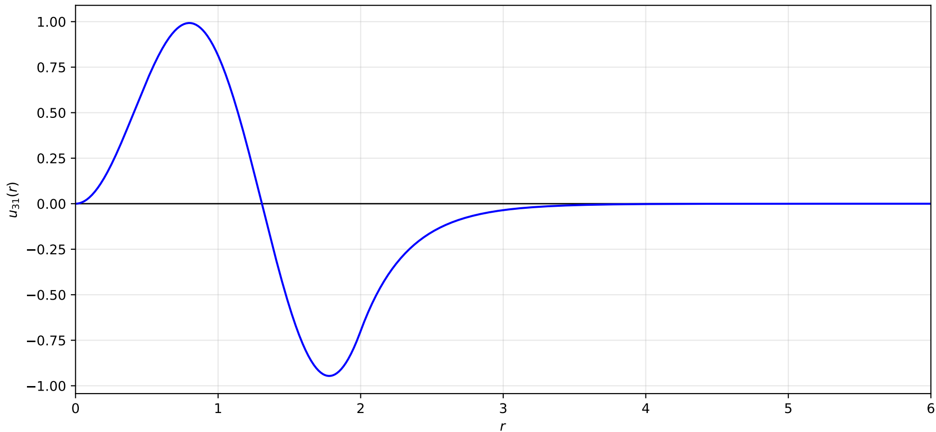
Reduced Radial Wave Function: n = 3, \ell = 1
