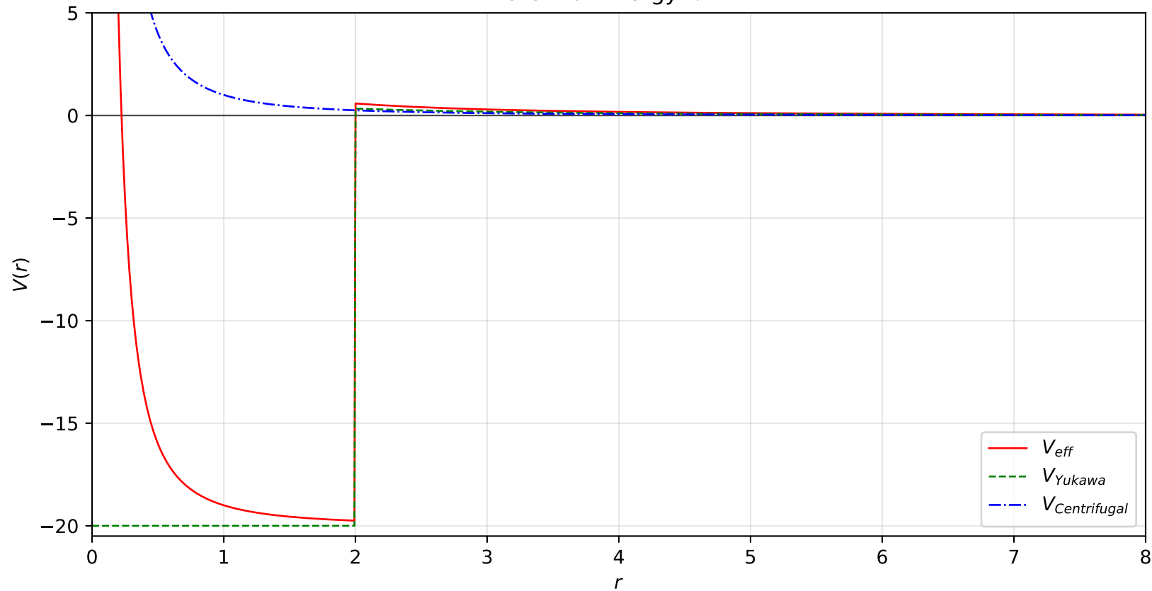
Potential Energy: \ell = 1
