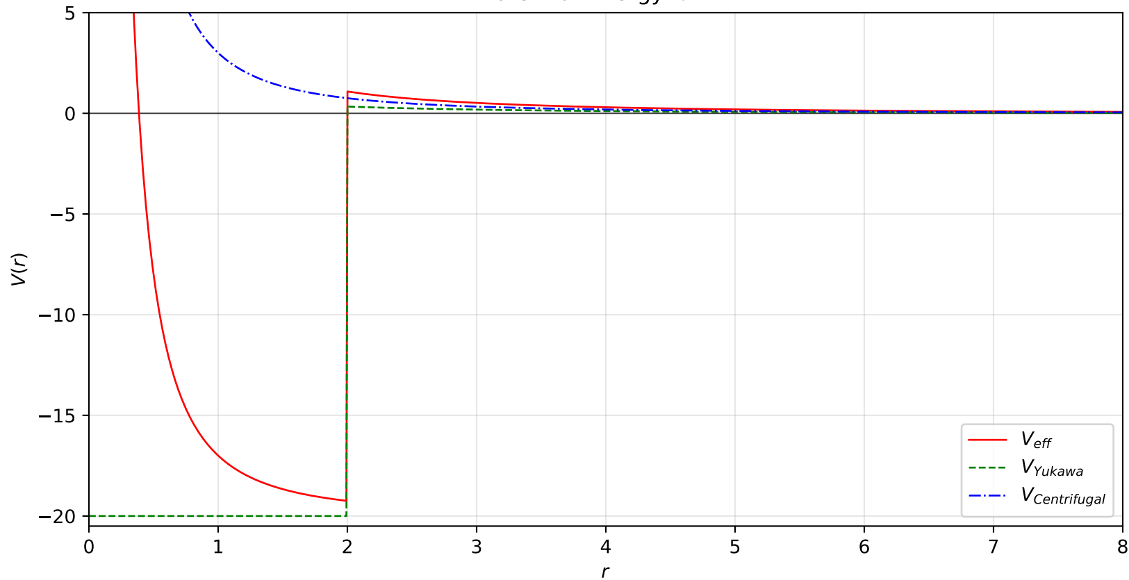
Potential Energy: \ell = 2
