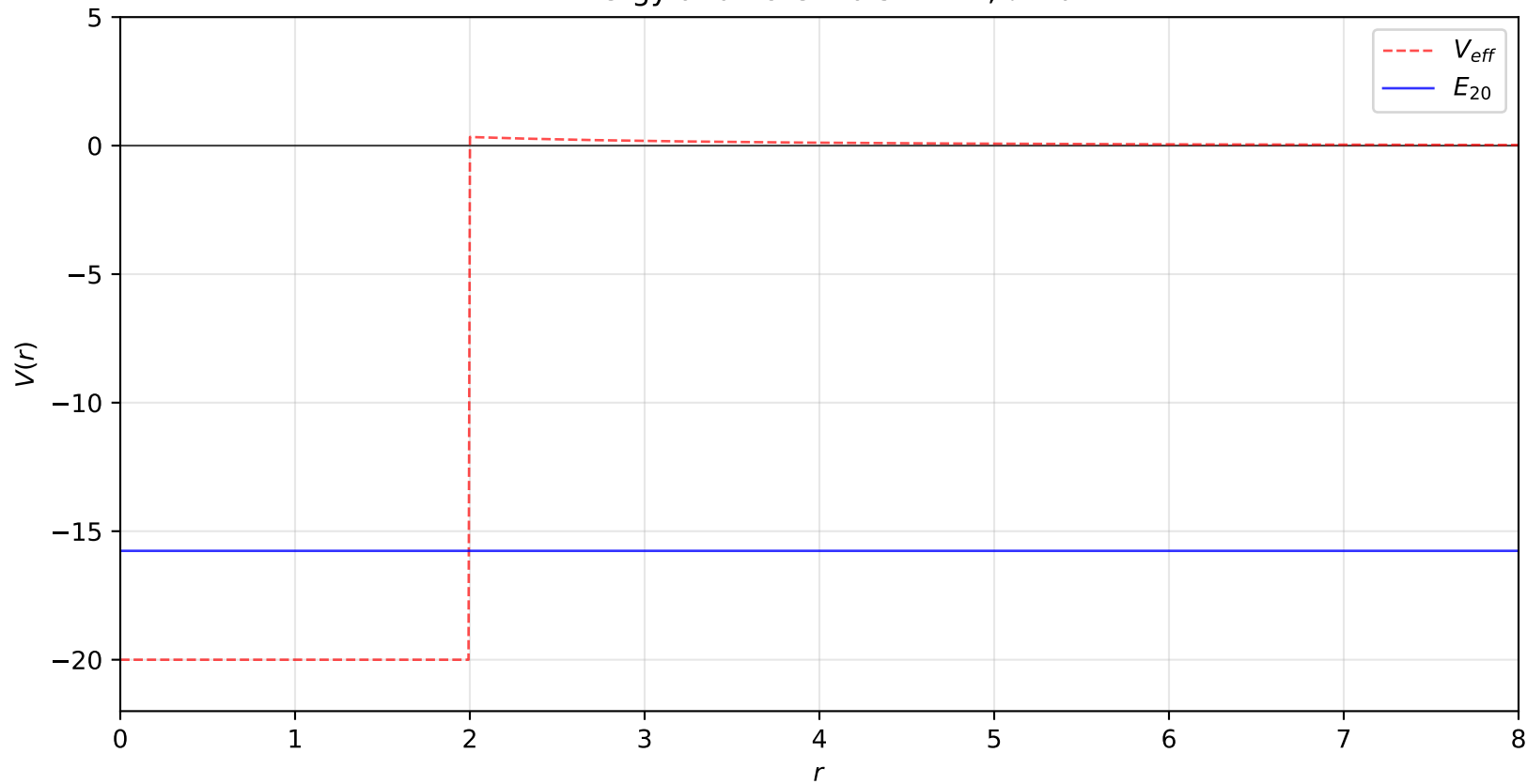
Energy and Potentials: n = 2, \ell = 0
