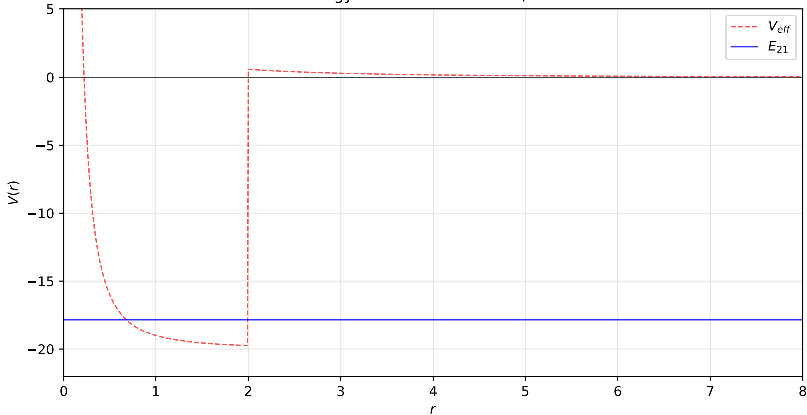
Energy and Potentials: n = 2, \ell = 1
