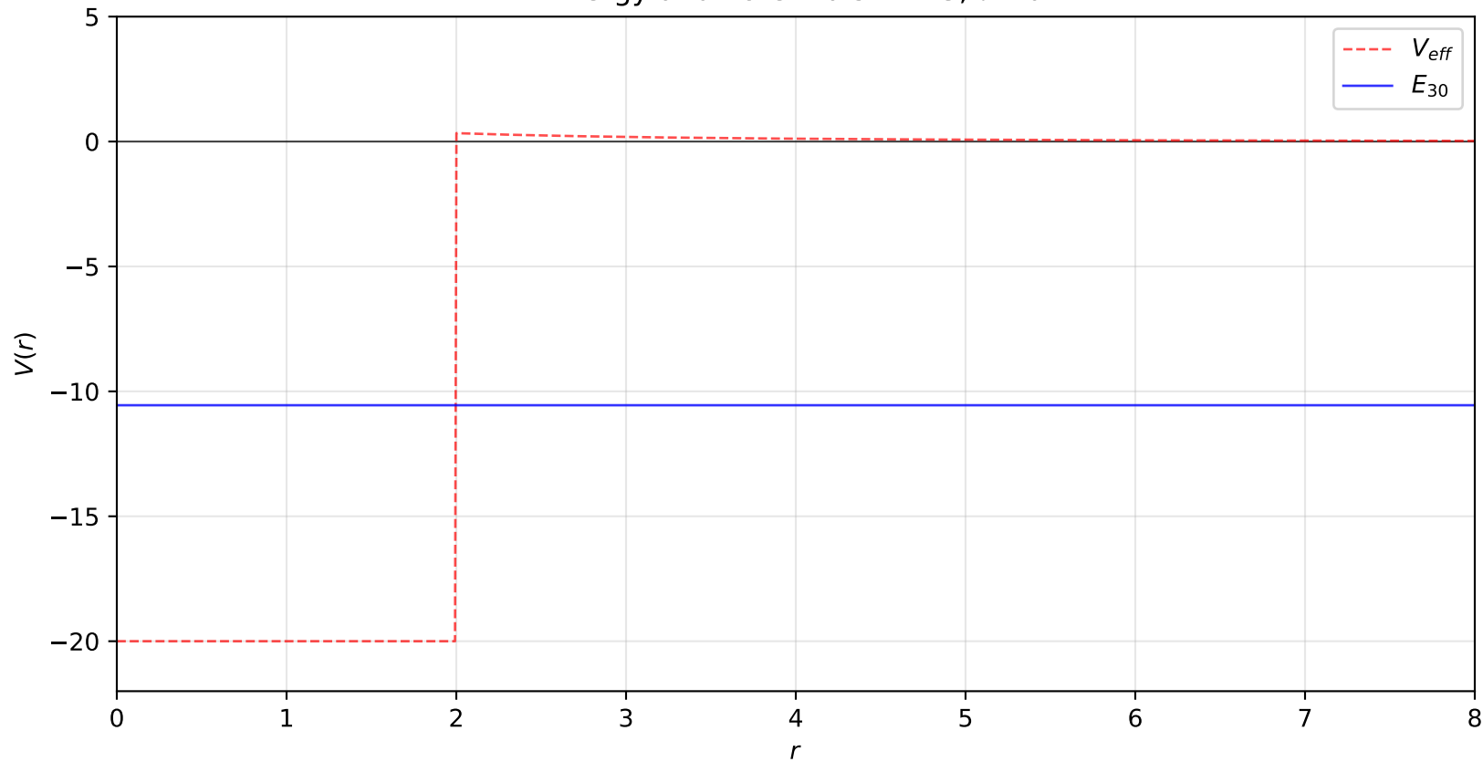
Energy and Potentials: n = 3, \ell = 0
