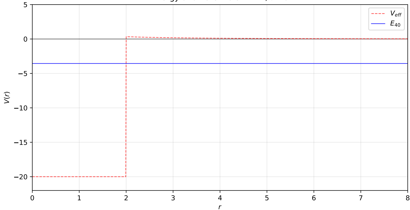
Energy and Potentials: n = 4, \ell = 0
