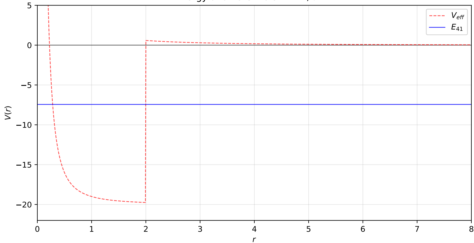
Energy and Potentials: n = 4, \ell = 1
