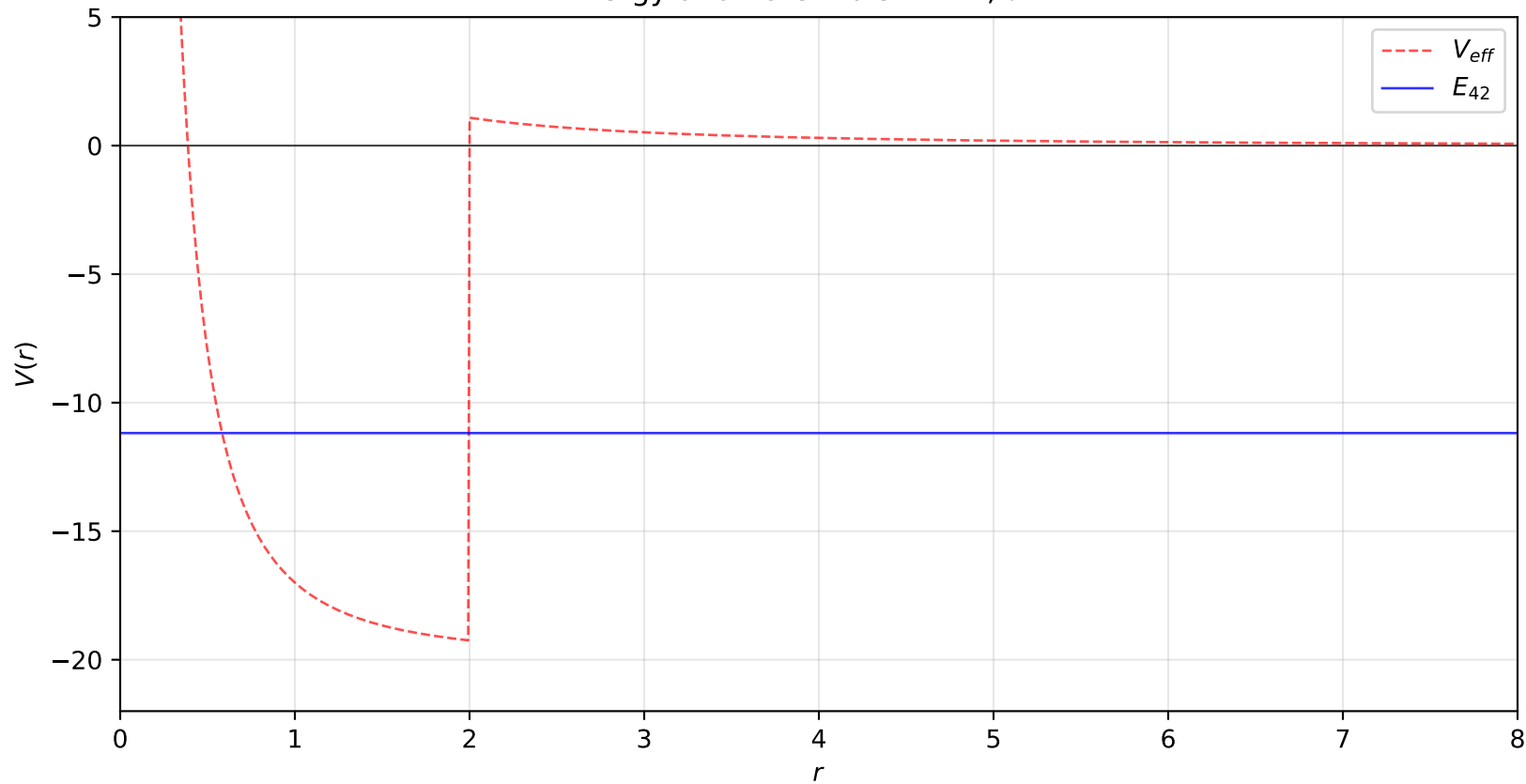
Energy and Potentials: n = 4, \ell = 2
