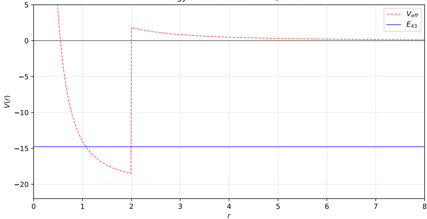
Energy and Potentials: n = 4, \ell = 3
