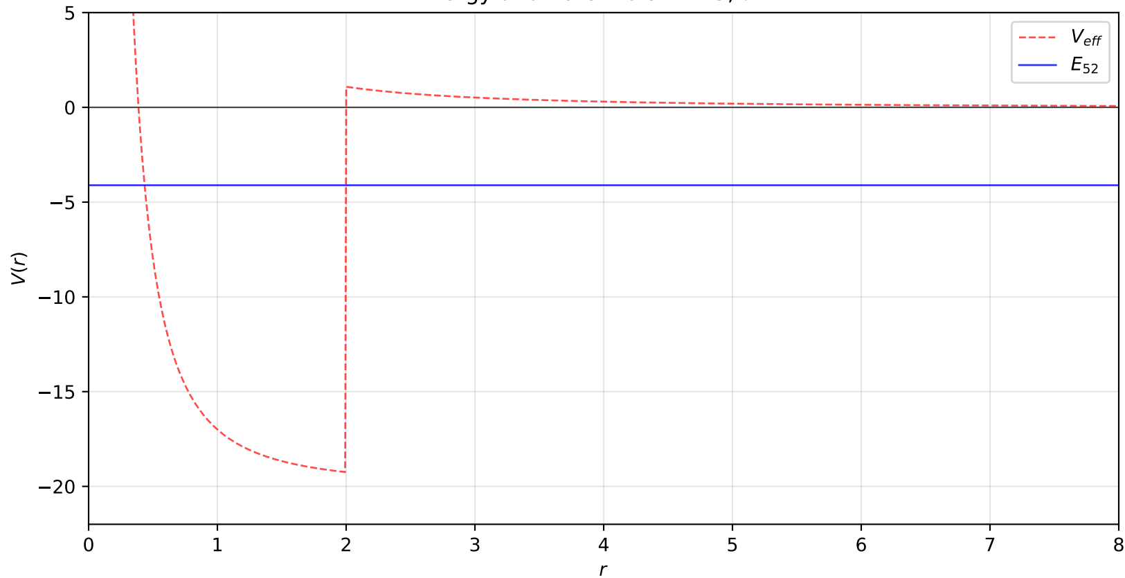
Energy and Potentials: n = 5, \ell = 2
