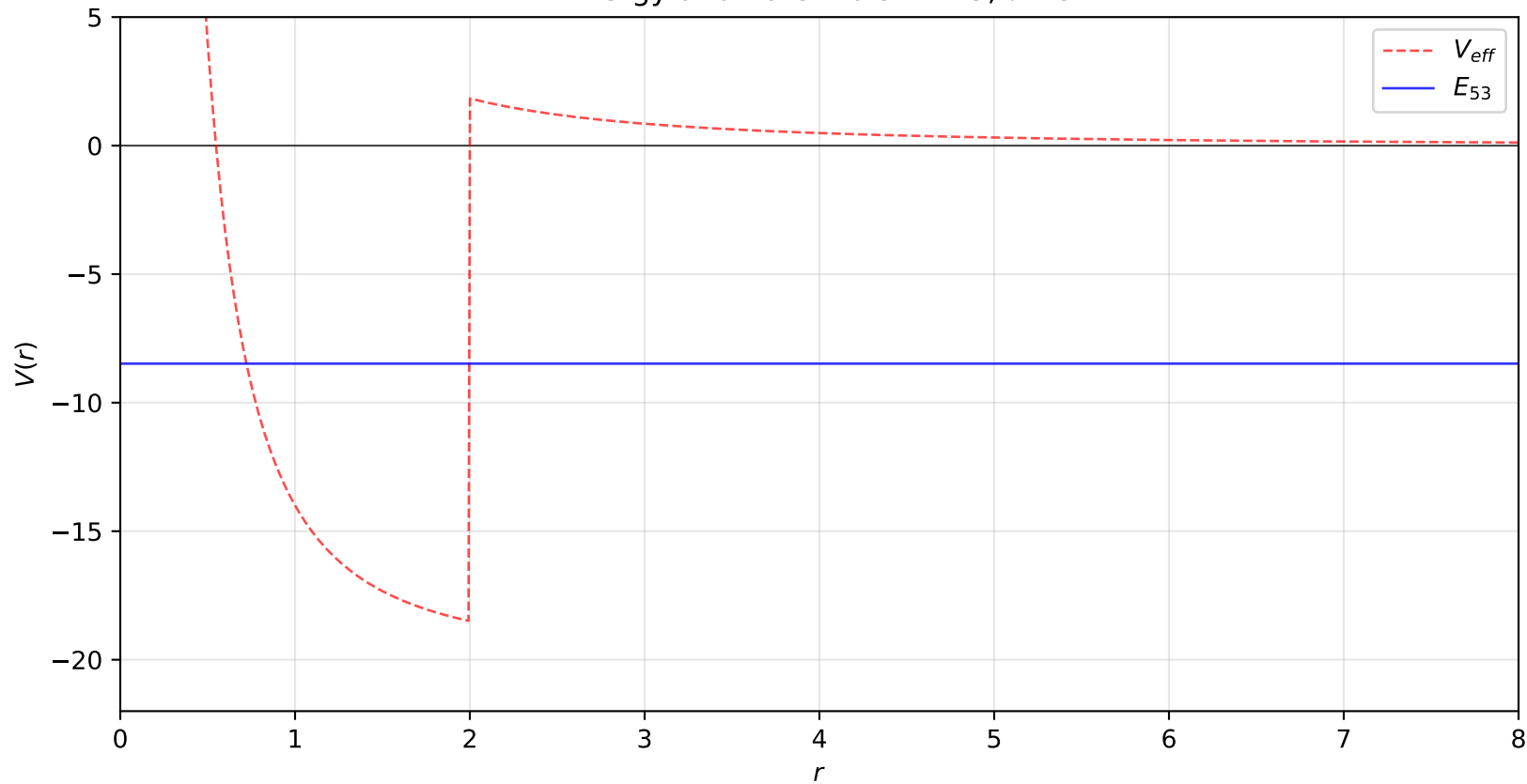
Energy and Potentials: n = 5, \ell = 3
