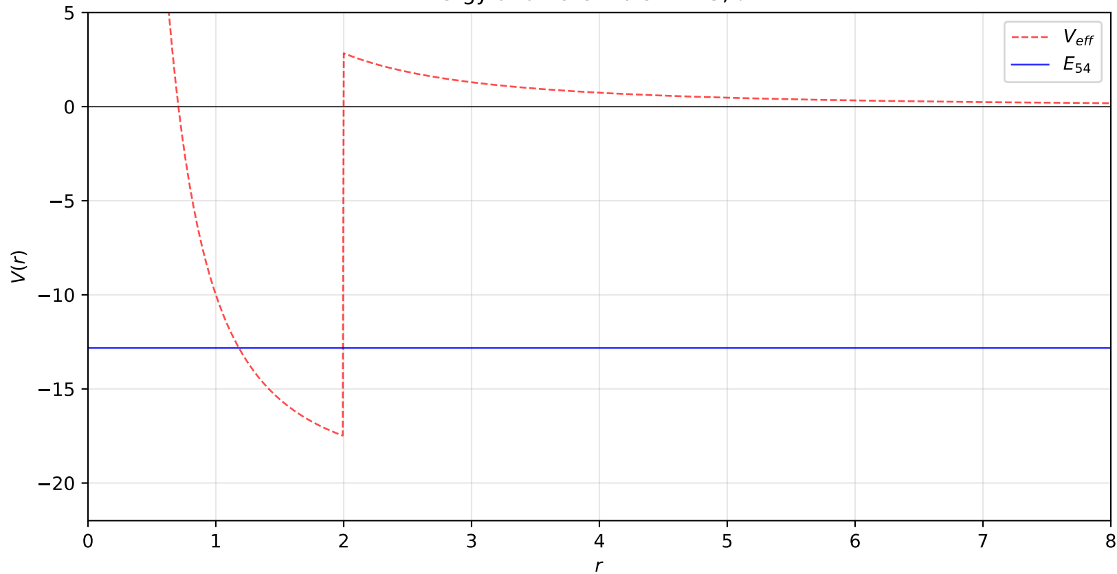
Energy and Potentials: n = 5, \ell = 4
