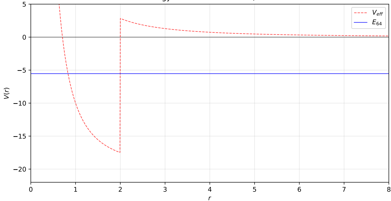
Energy and Potentials: n = 6, \ell = 4
