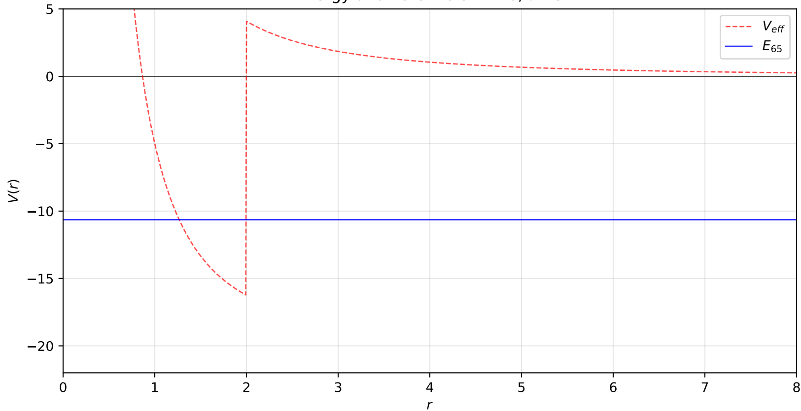
Energy and Potentials: n = 6, \ell = 5
