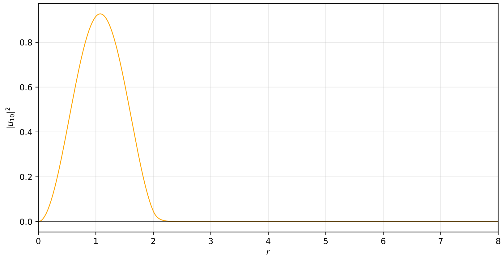
Probability Density: n = 1, \ell = 0
