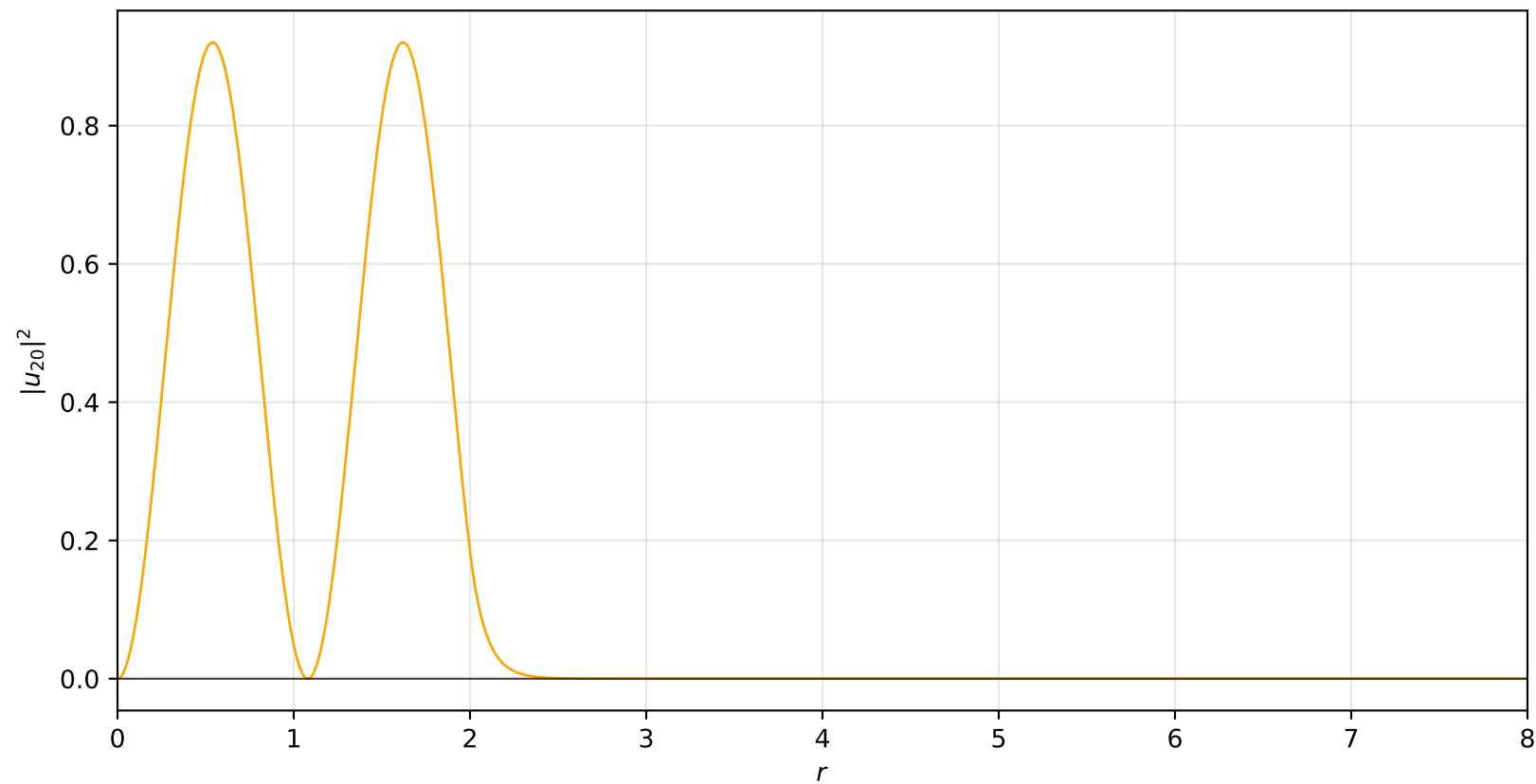
Probability Density: n = 2, \ell = 0
