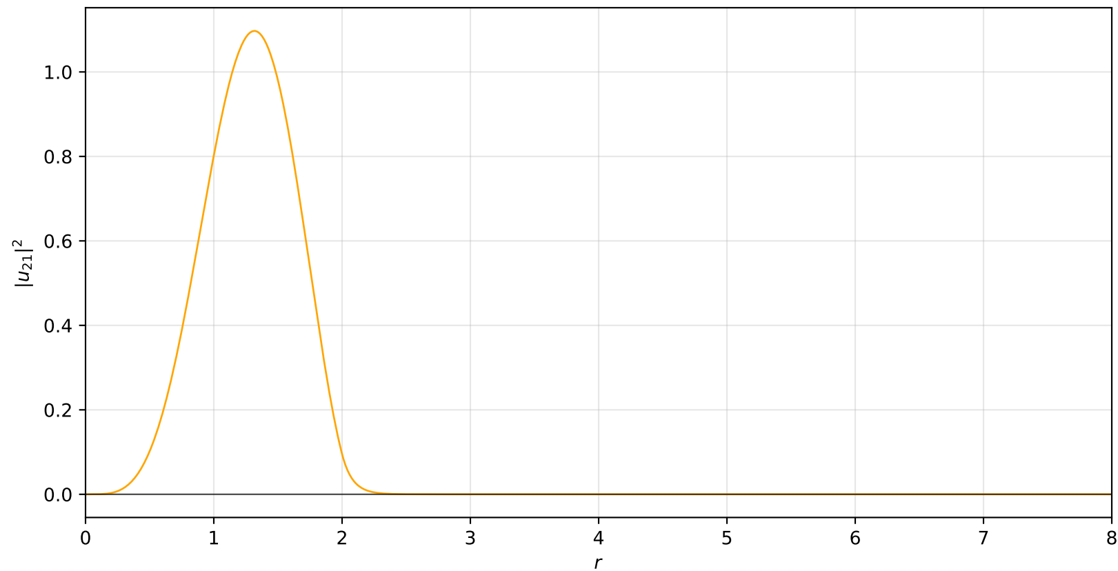
Probability Density: n = 2, \ell = 1
