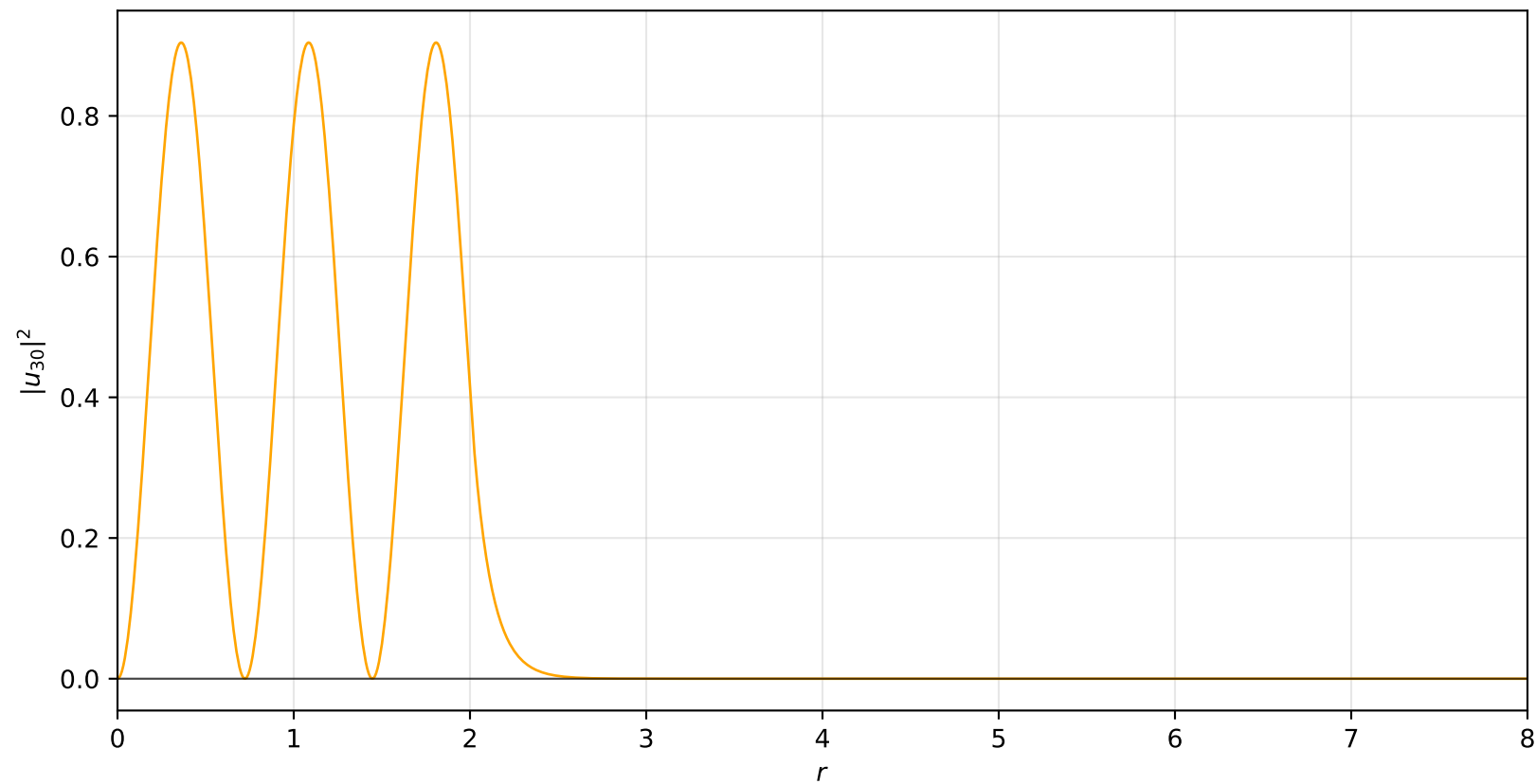
Probability Density: n = 3, \ell = 0
