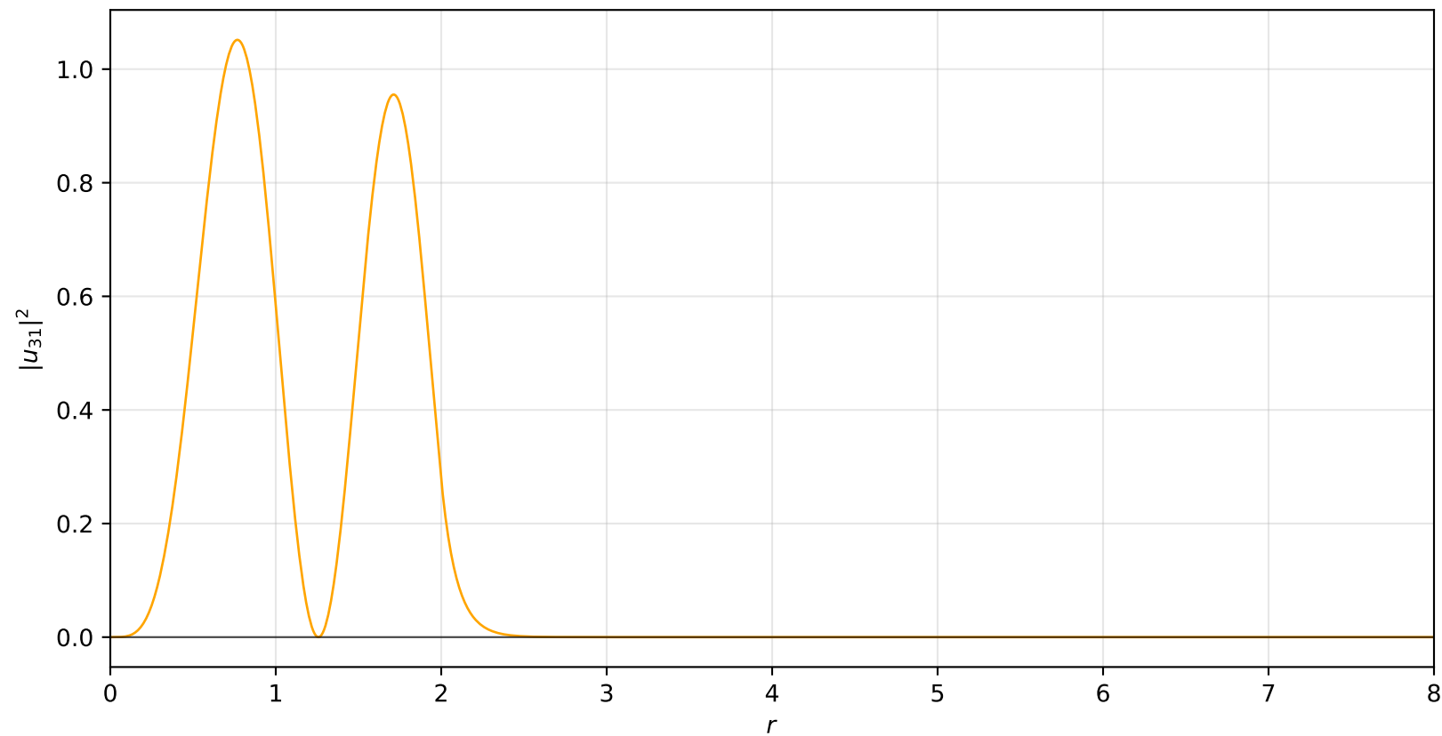
Probability Density: n = 3, \ell = 1
