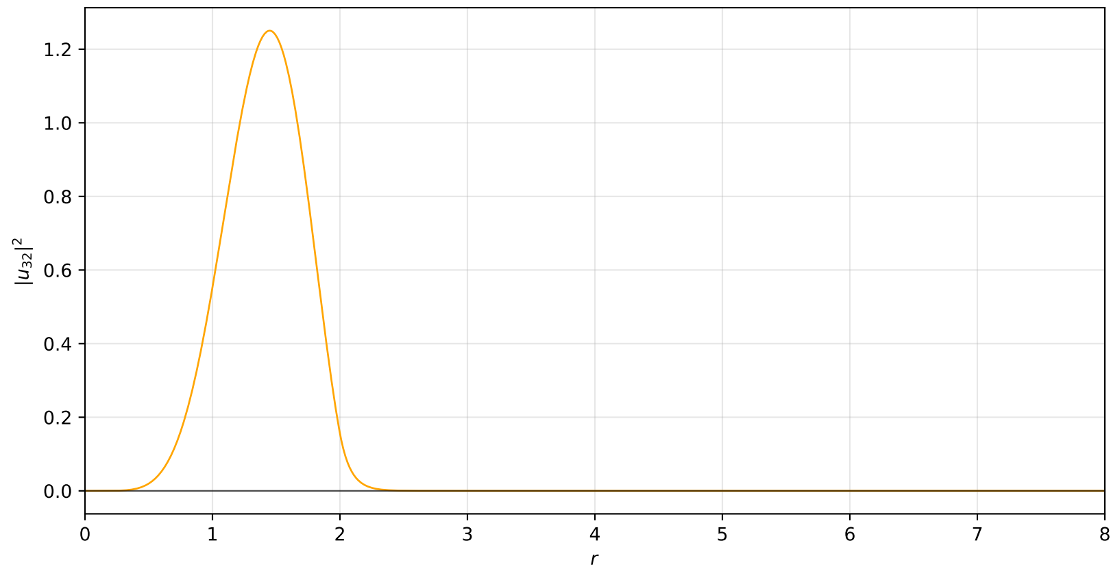
Probability Density: n = 3, \ell = 2
