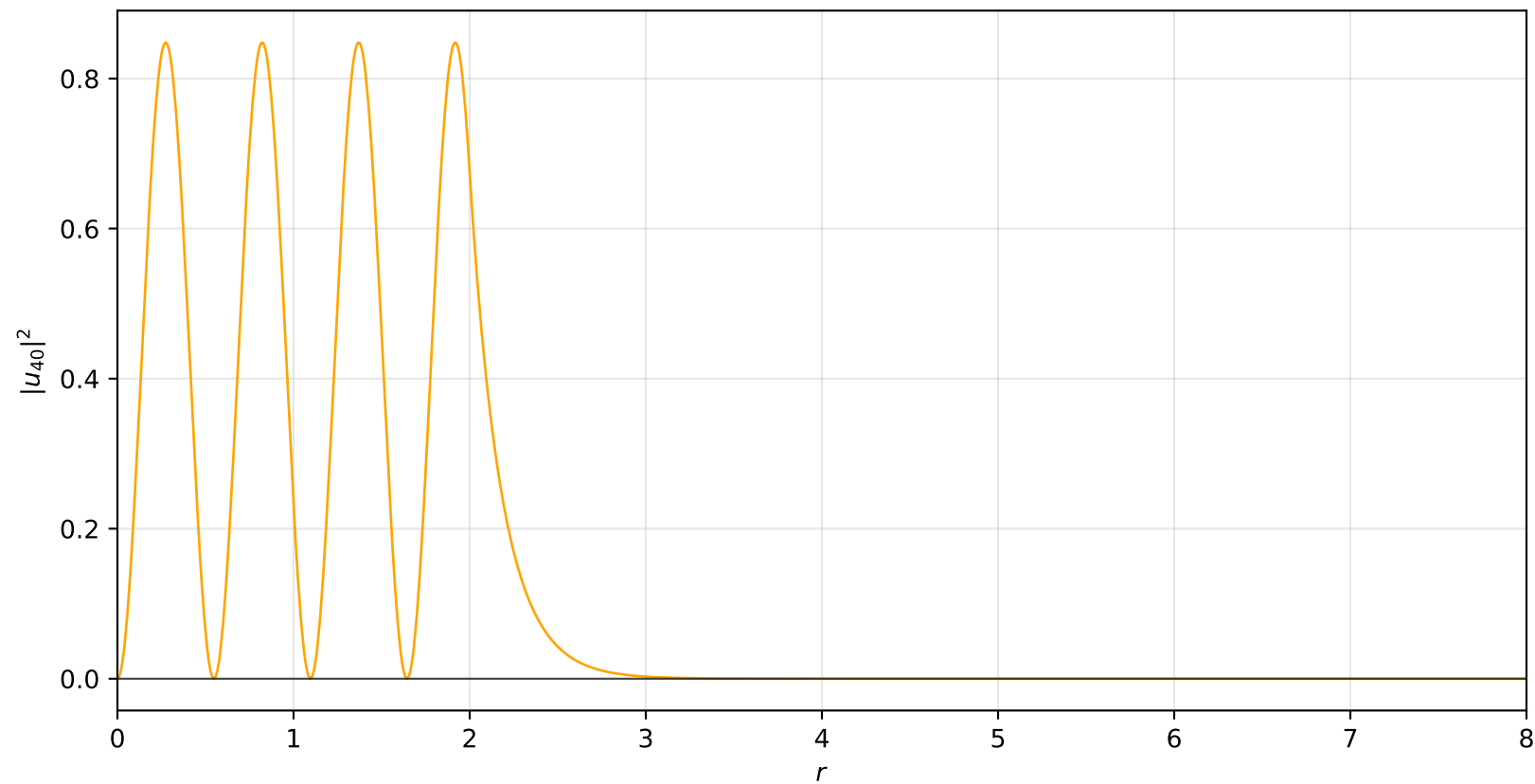
Probability Density: n = 4, \ell = 0
