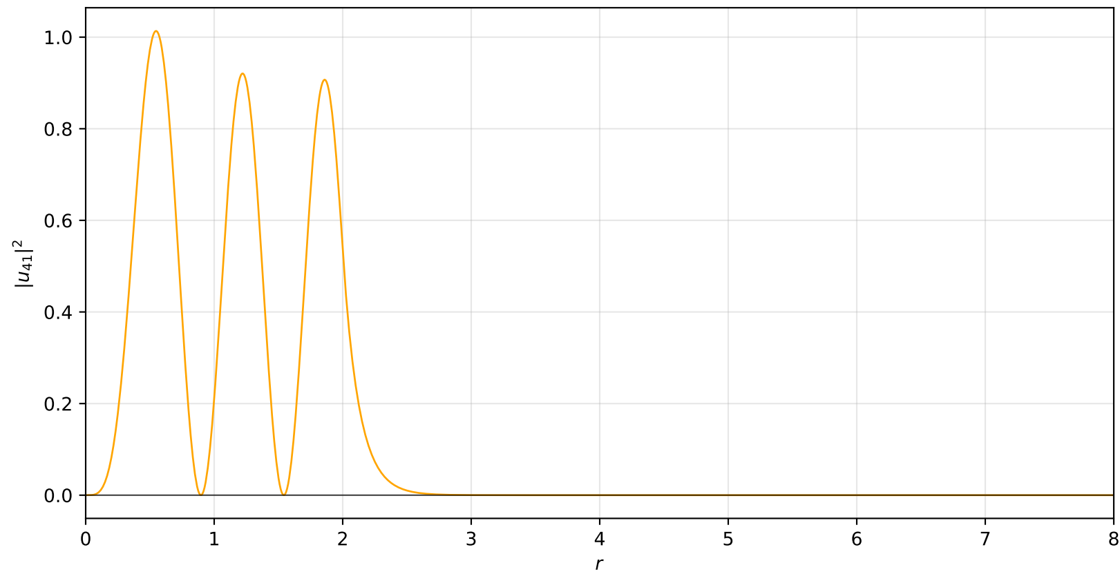
Probability Density: n = 4, \ell = 1
