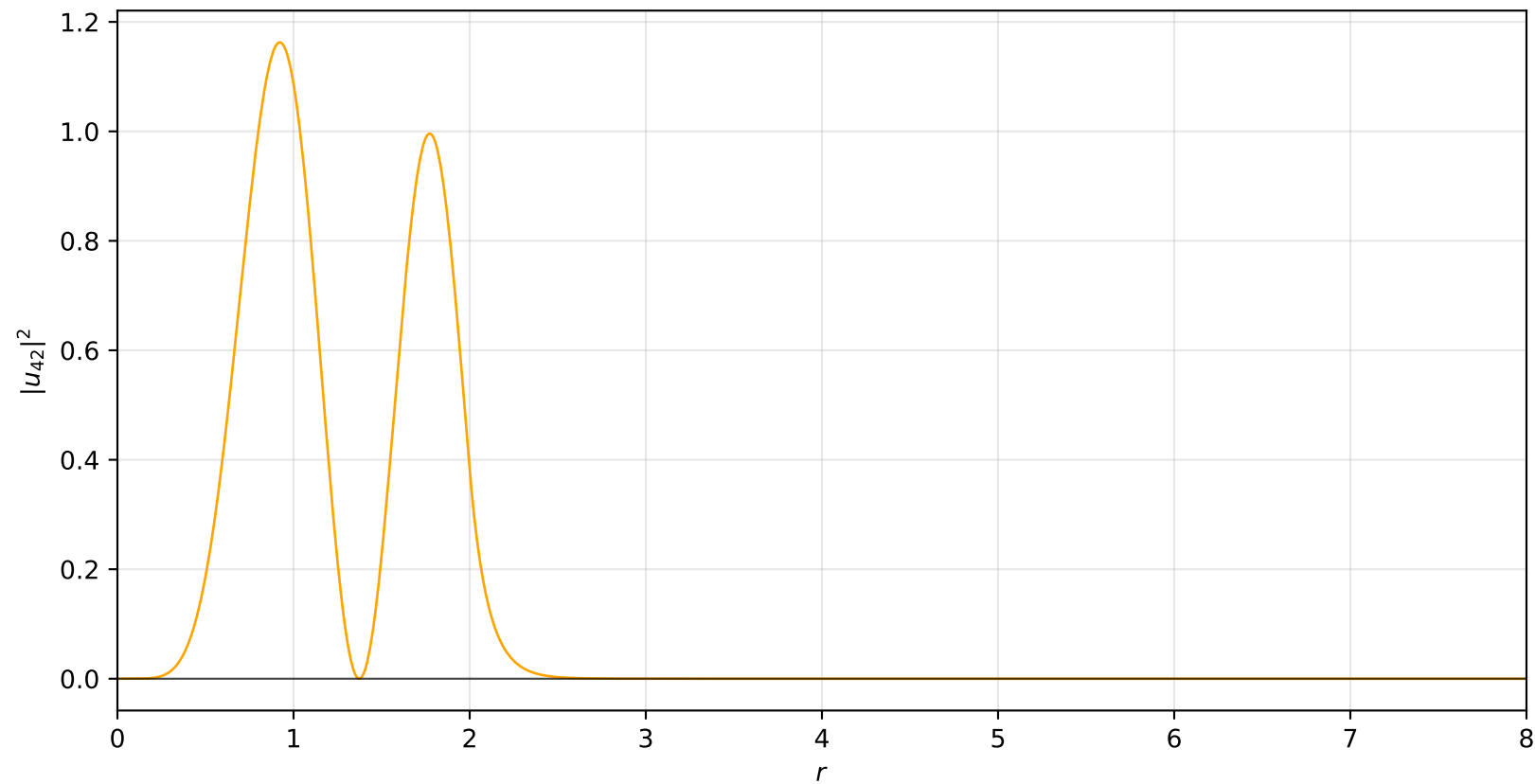
Probability Density: n = 4, \ell = 2
