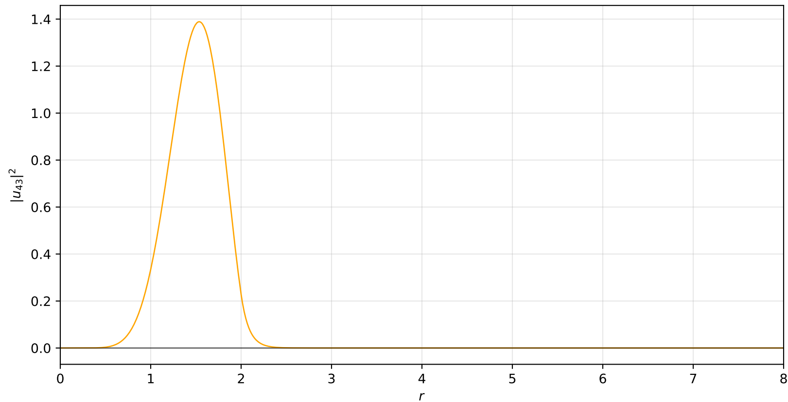
Probability Density: n = 4, \ell = 3
