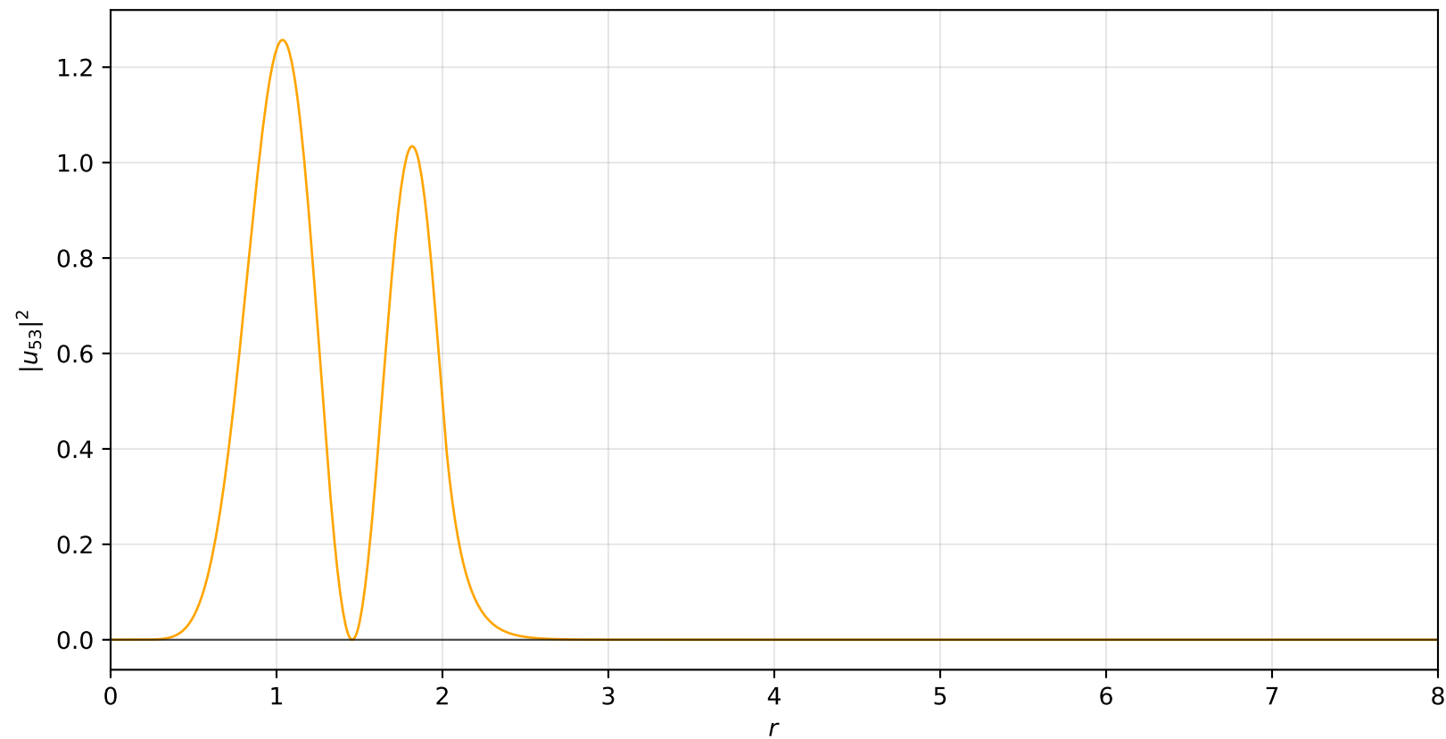
Probability Density: n = 5, \ell = 3
