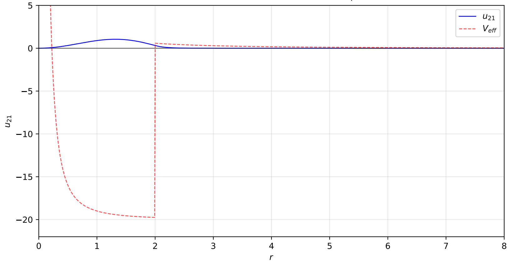
Reduced Radial Wave Function: n = 2, \ell = 1
