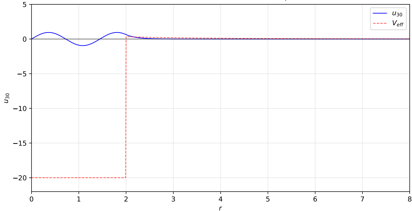
Reduced Radial Wave Function: n = 3, \ell = 0
