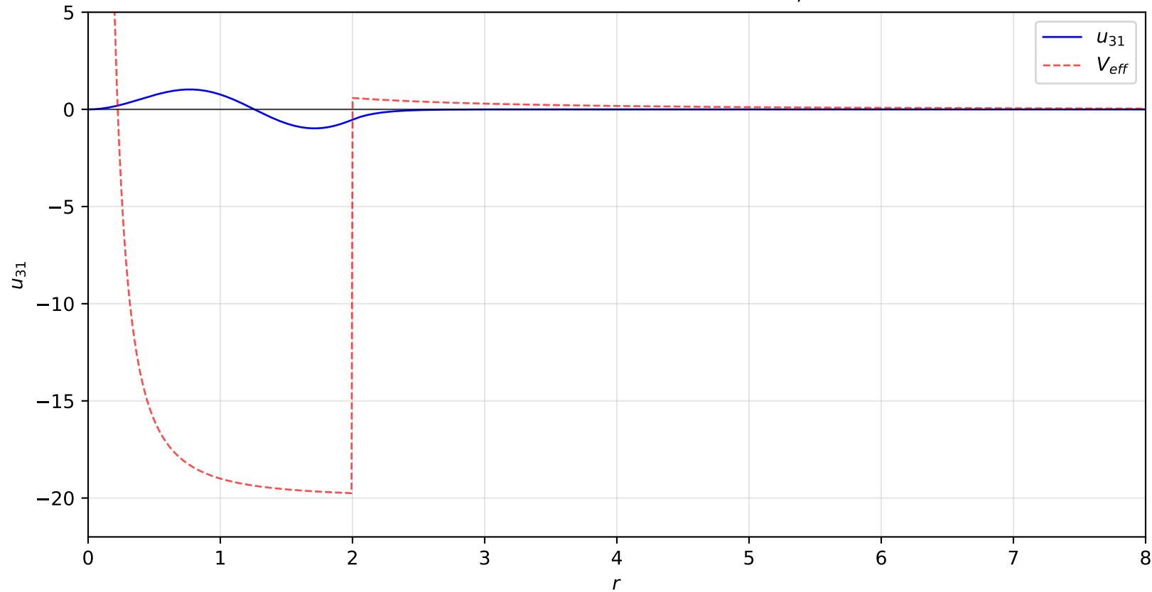
Reduced Radial Wave Function: n = 3, \ell = 1
