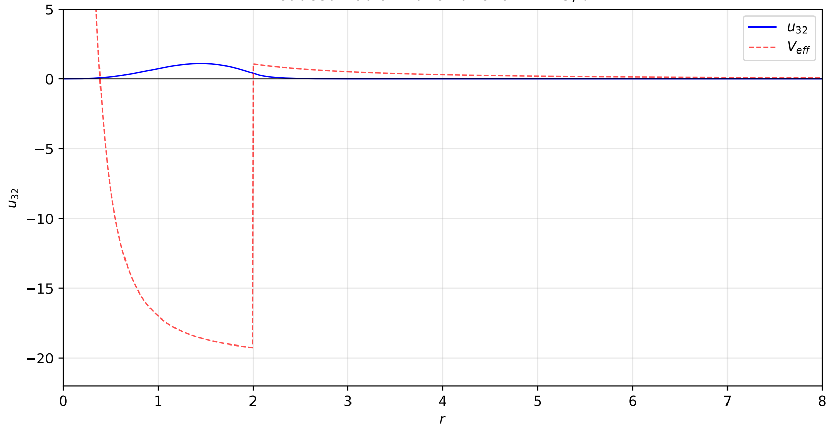
Reduced Radial Wave Function: n = 3, \ell = 2
