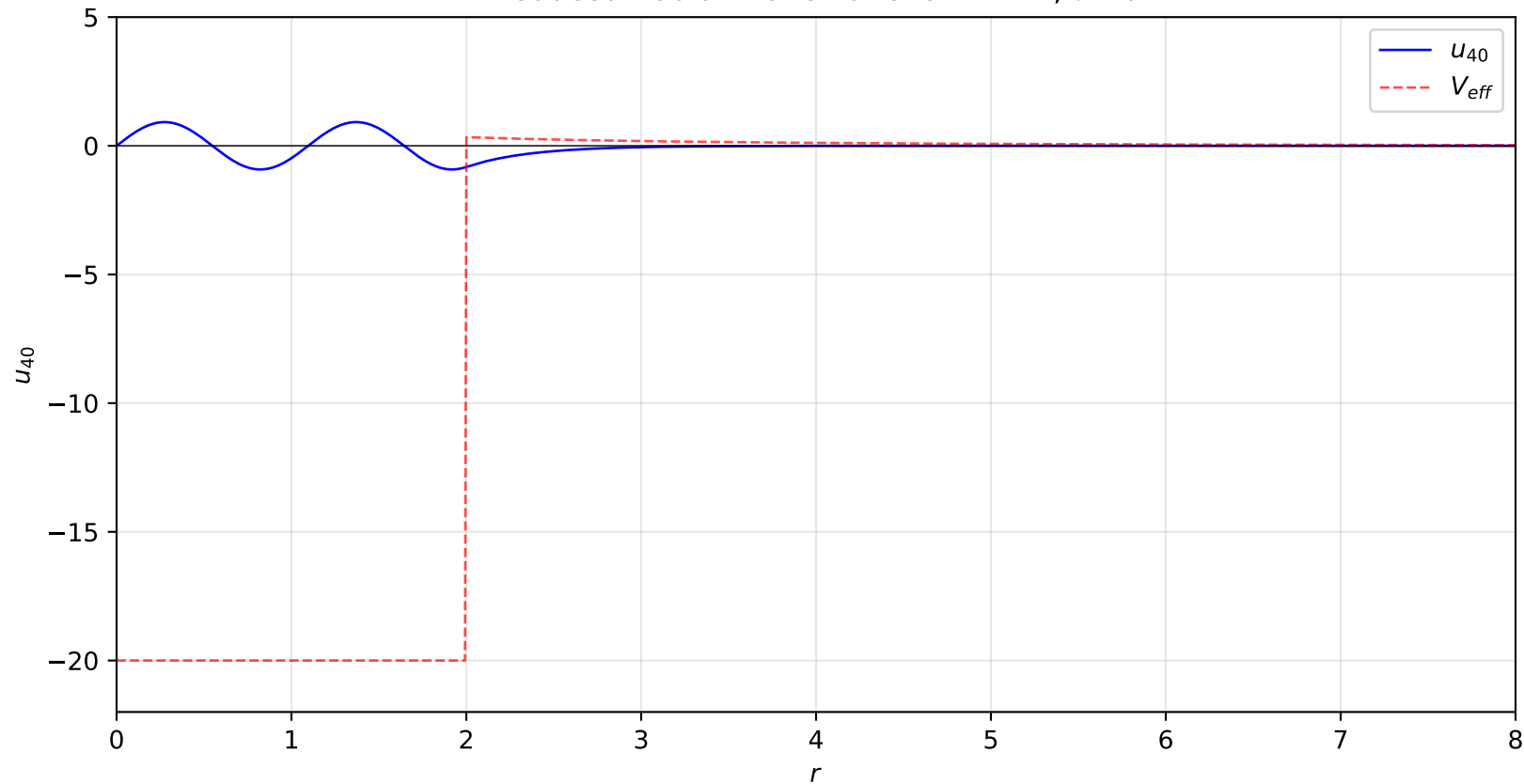
Reduced Radial Wave Function: n = 4, \ell = 0
