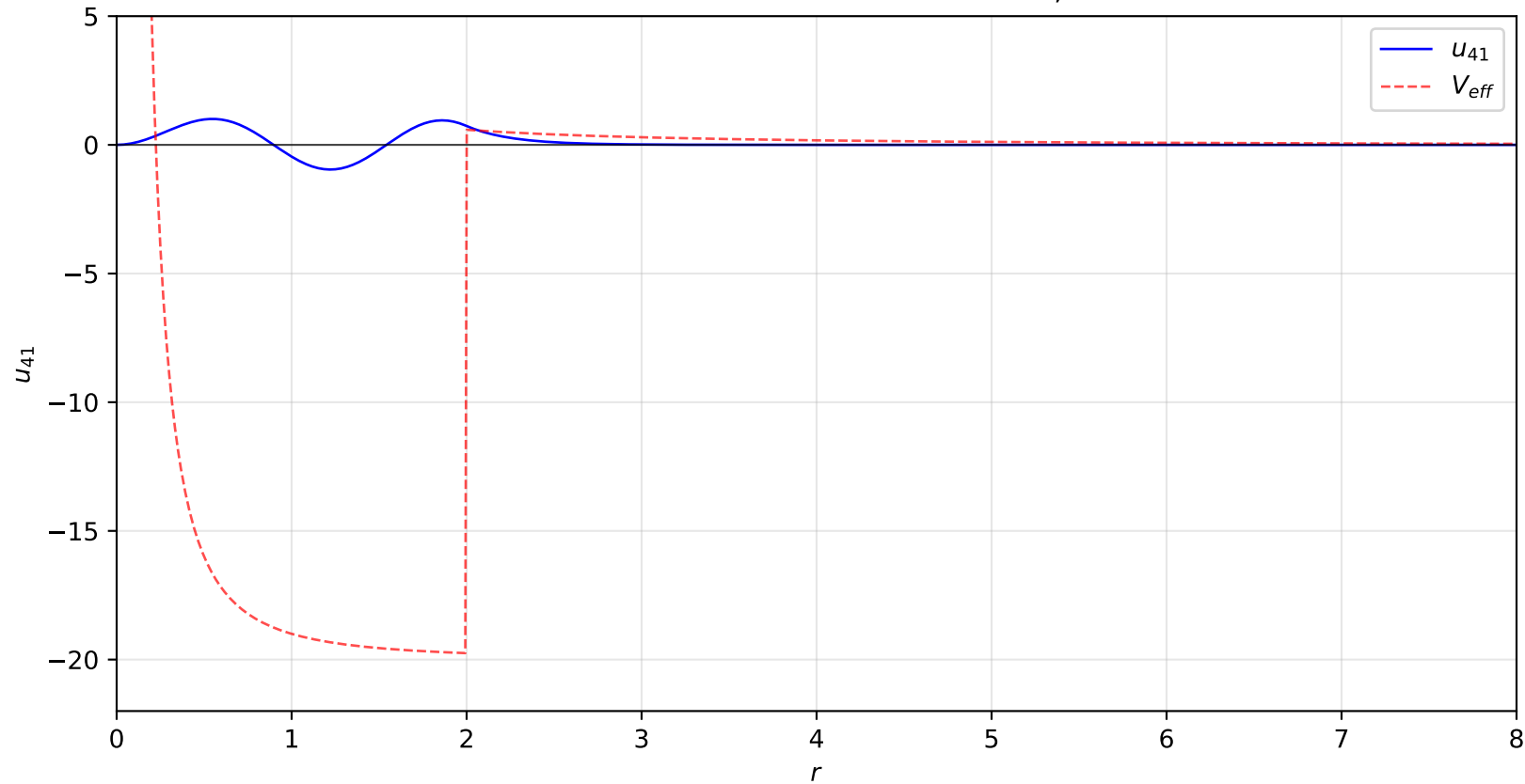
Reduced Radial Wave Function: n = 4, \ell = 1
