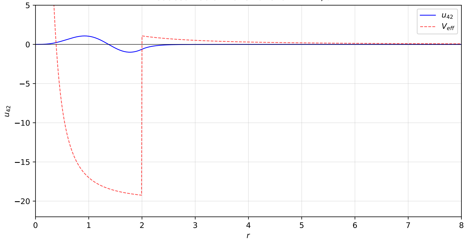
Reduced Radial Wave Function: n = 4, \ell = 2
