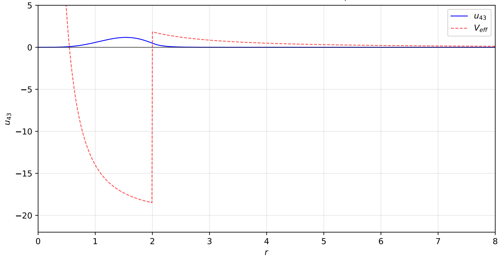
Reduced Radial Wave Function: n = 4, \ell = 3
