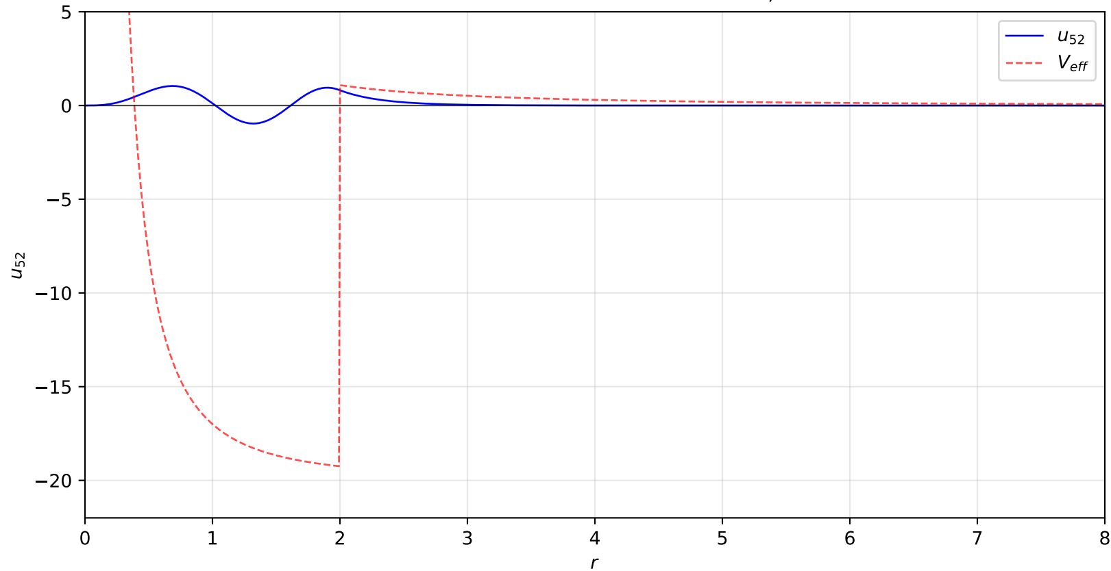
Reduced Radial Wave Function: n = 5, \ell = 2
