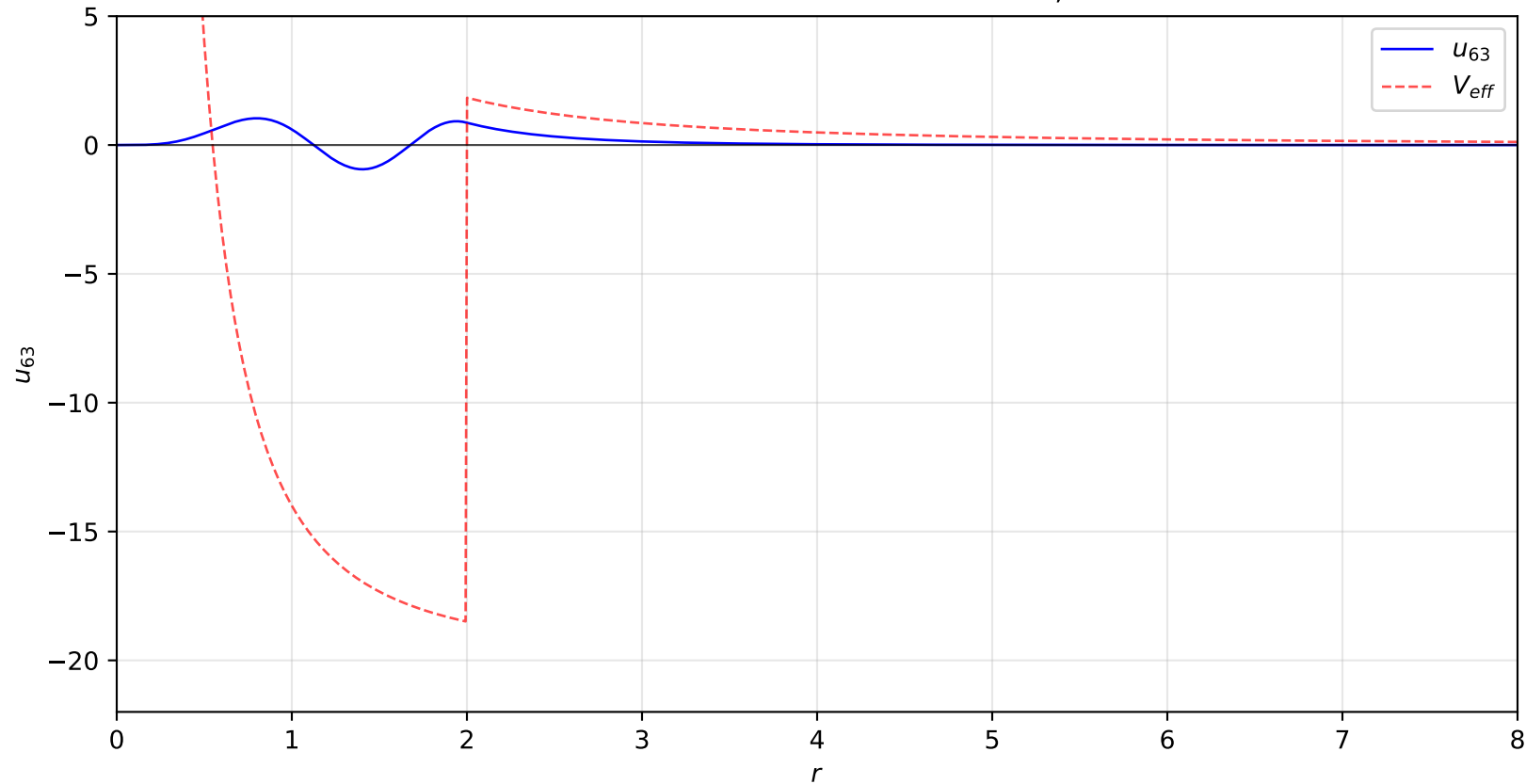
Reduced Radial Wave Function: n = 6, \ell = 3
