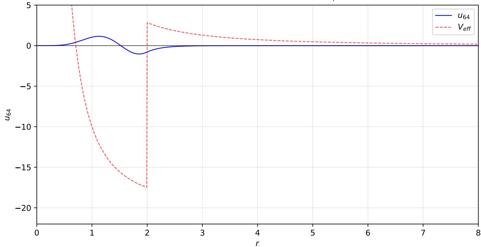
Reduced Radial Wave Function: n = 6, \ell = 4
