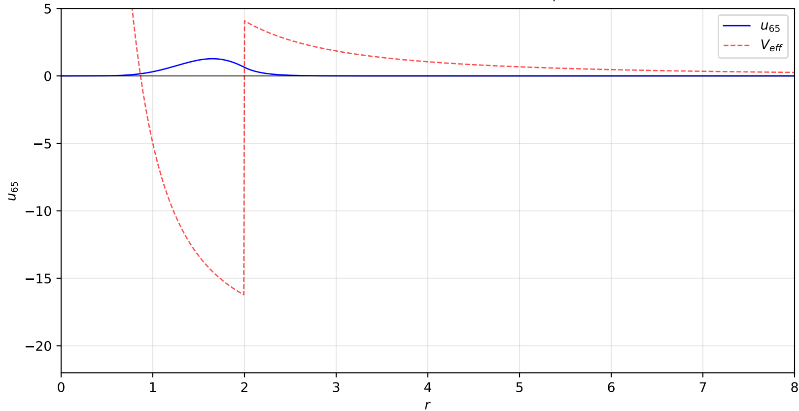
Reduced Radial Wave Function: n = 6, \ell = 5
