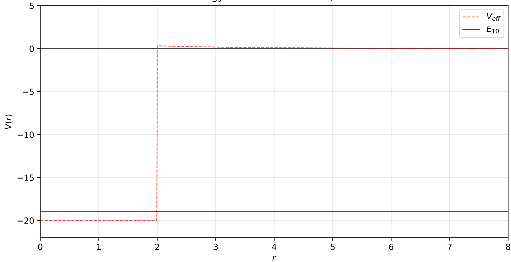
Energy and Potentials: n = 1, \ell = 0
