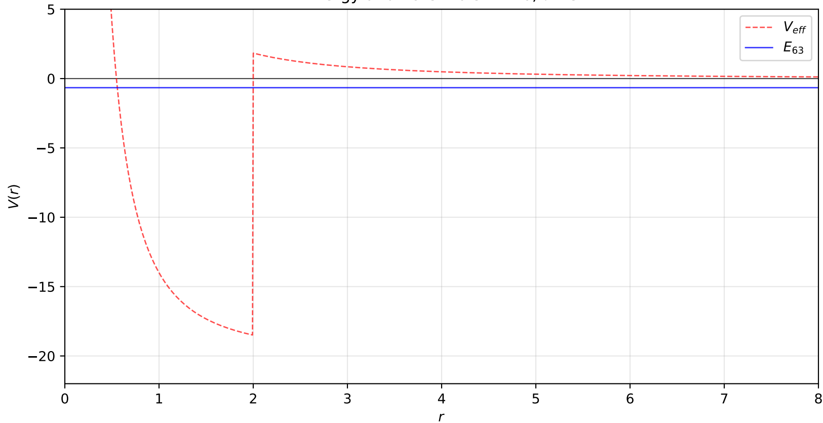
Energy and Potentials: n = 6, \ell = 3
