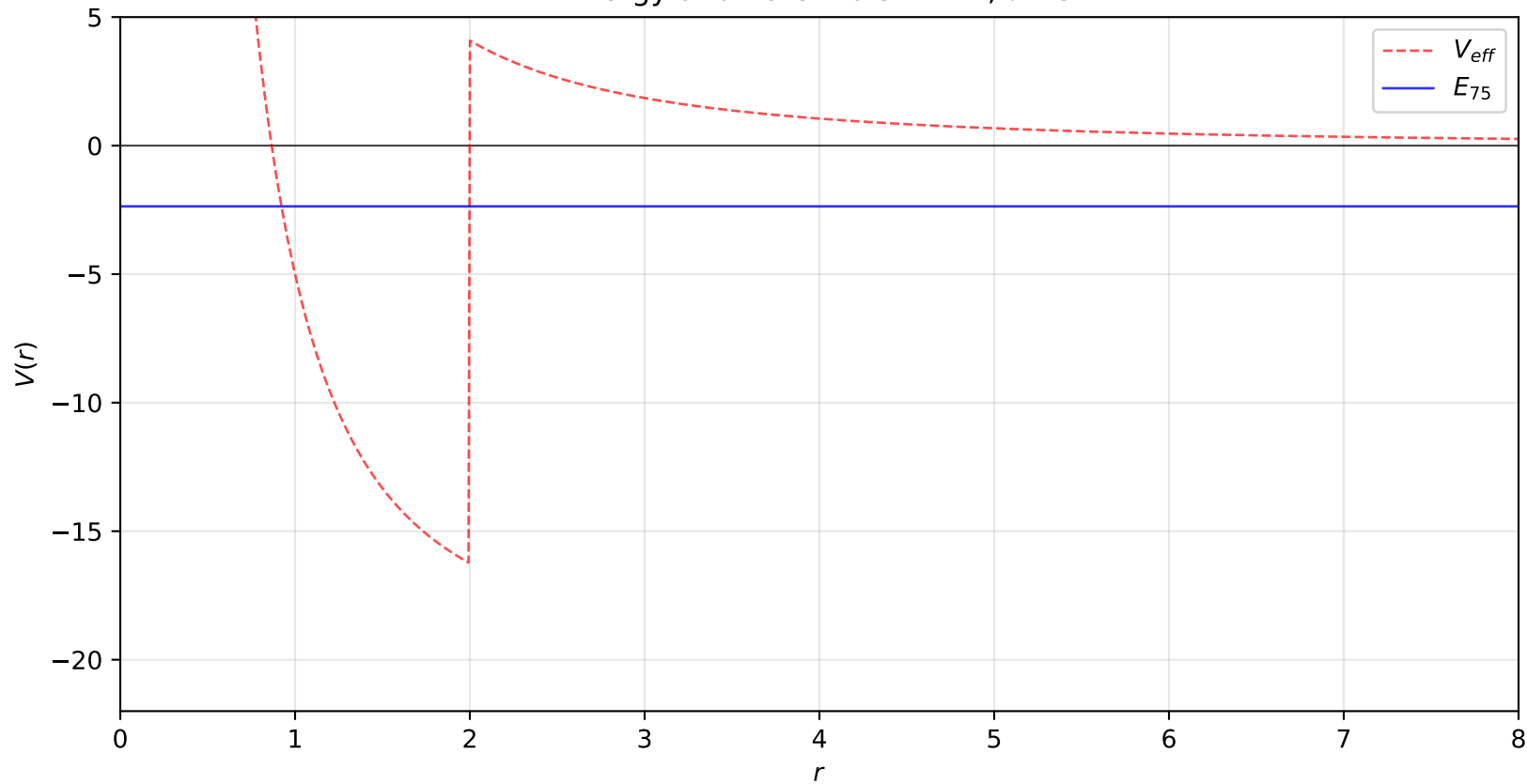
Energy and Potentials: n = 7, \ell = 5
