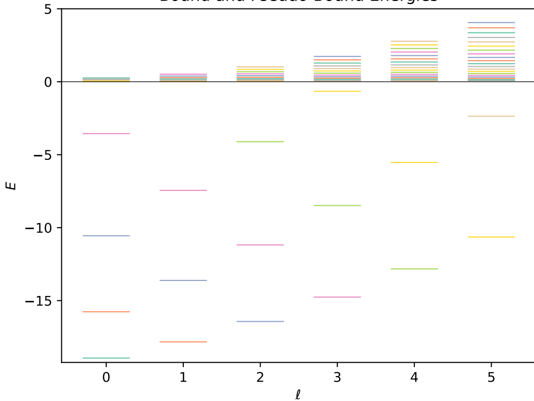
Bound and Pseudo-Bound Energies
