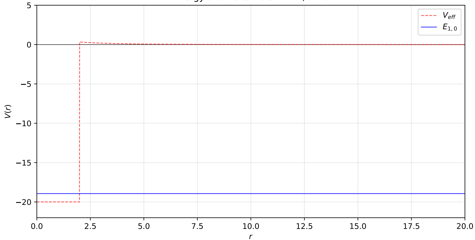
Energy and Potentials: n = 1, \ell = 0
