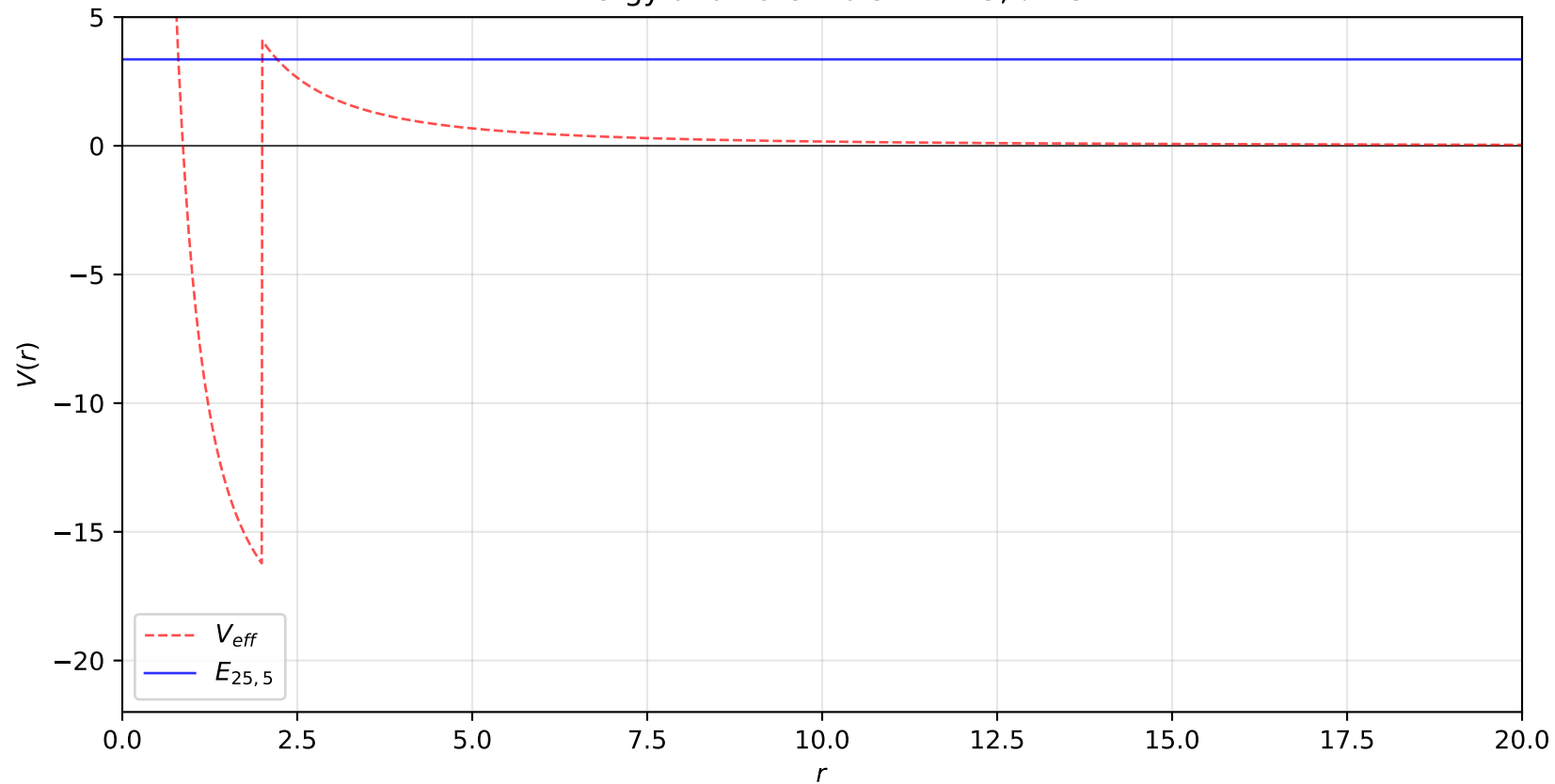
Energy and Potentials: n = 25, \ell = 5
