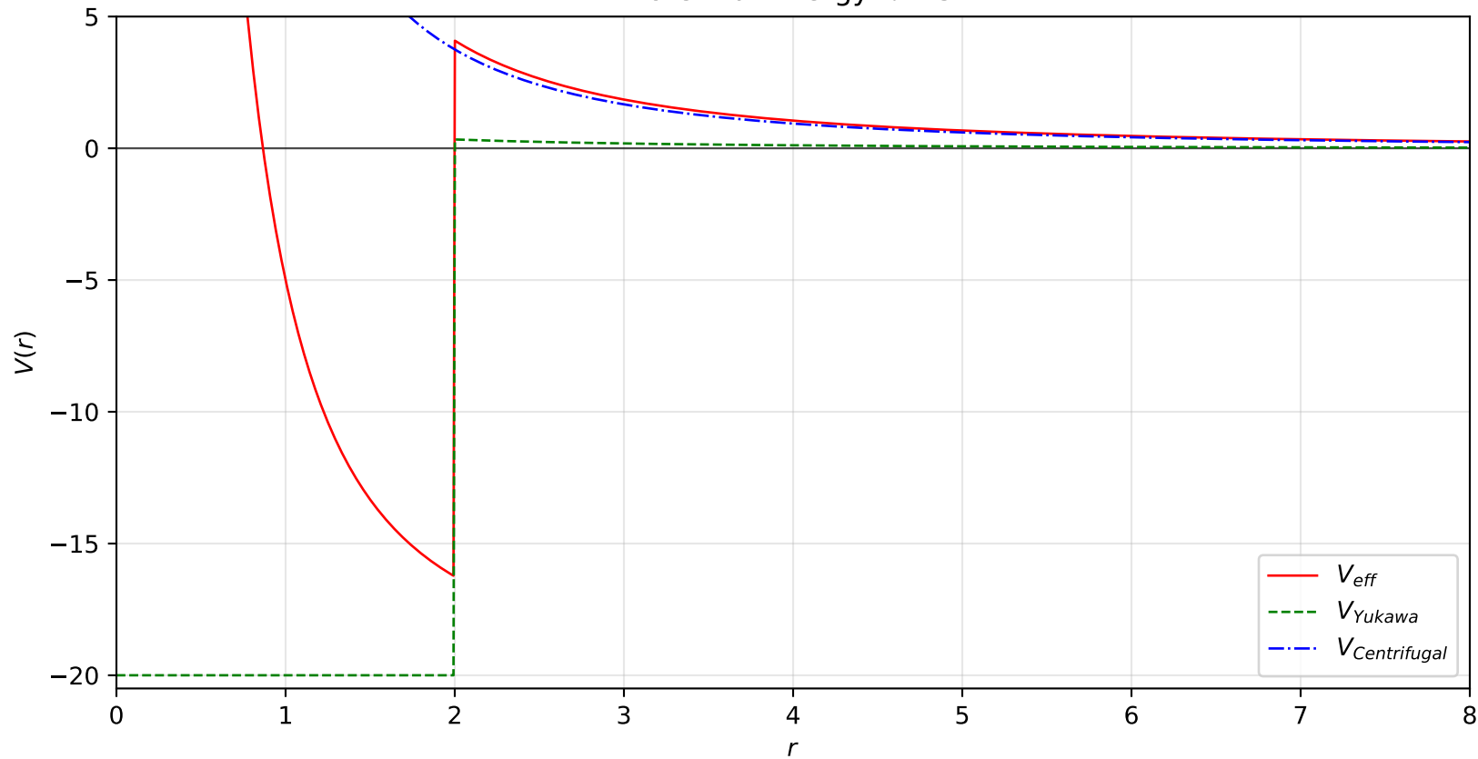
Potential Energy: \ell = 5
