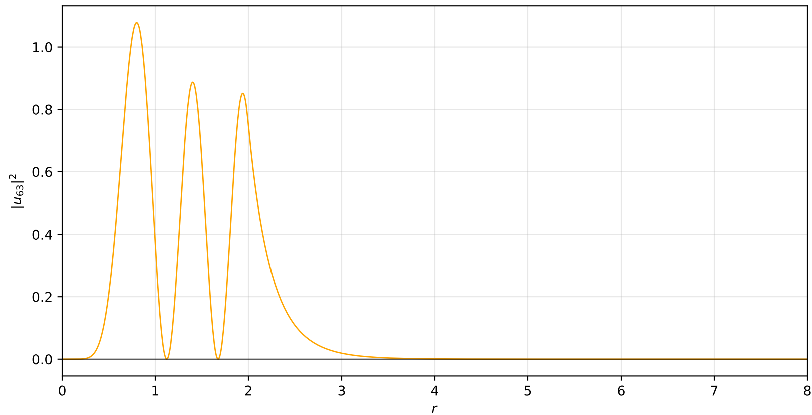
Probability Density: n = 6, \ell = 3
