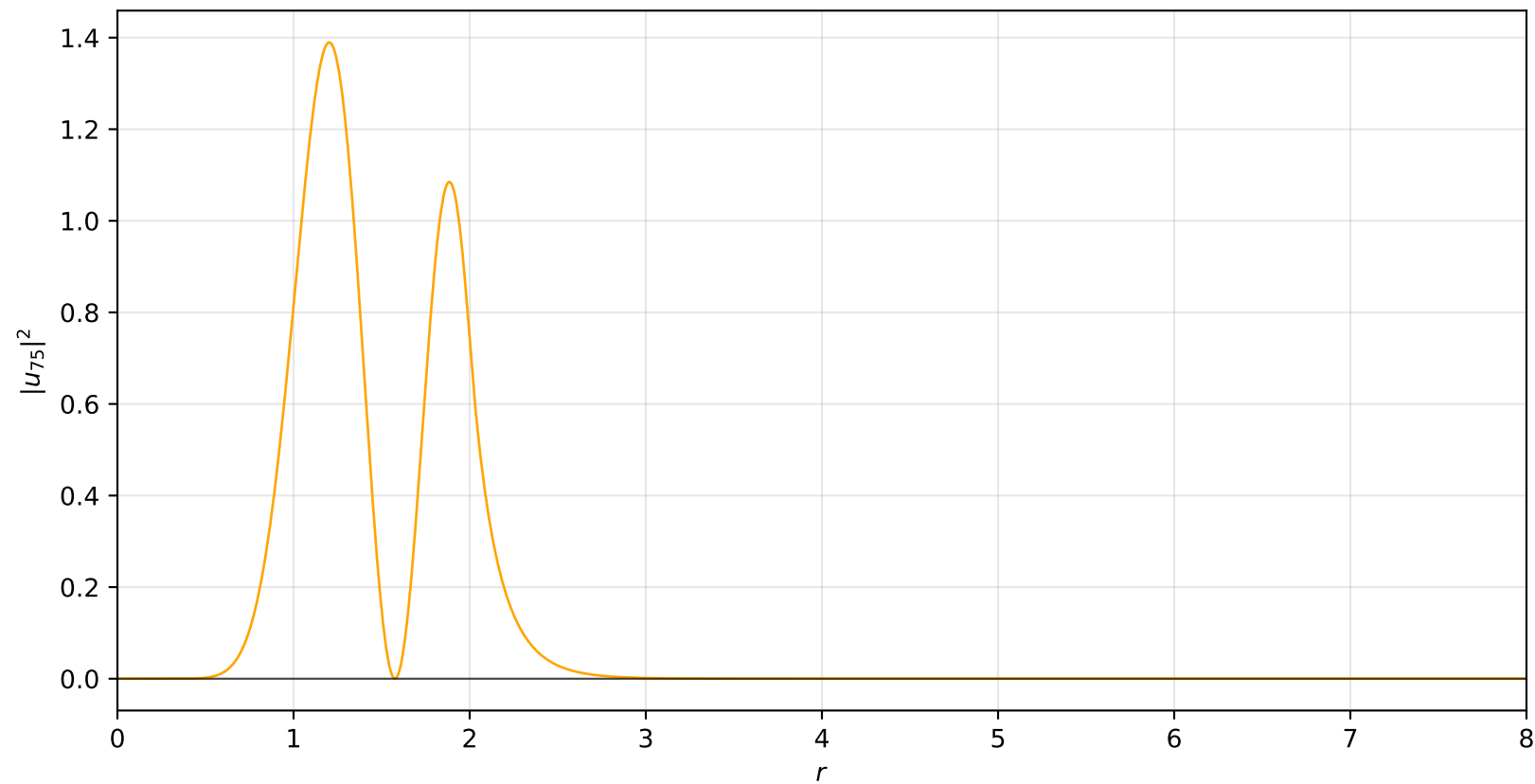
Probability Density: n = 7, \ell = 5
