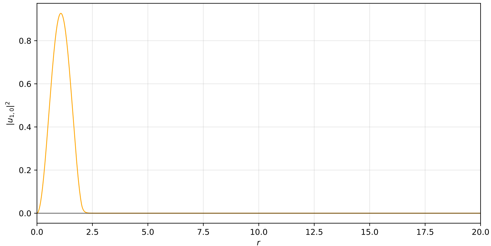
Probability Density: n = 1, \ell = 0
